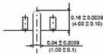
Detail Z
